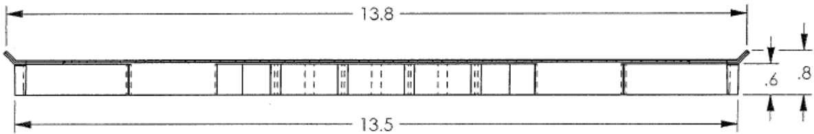
END VIEW
